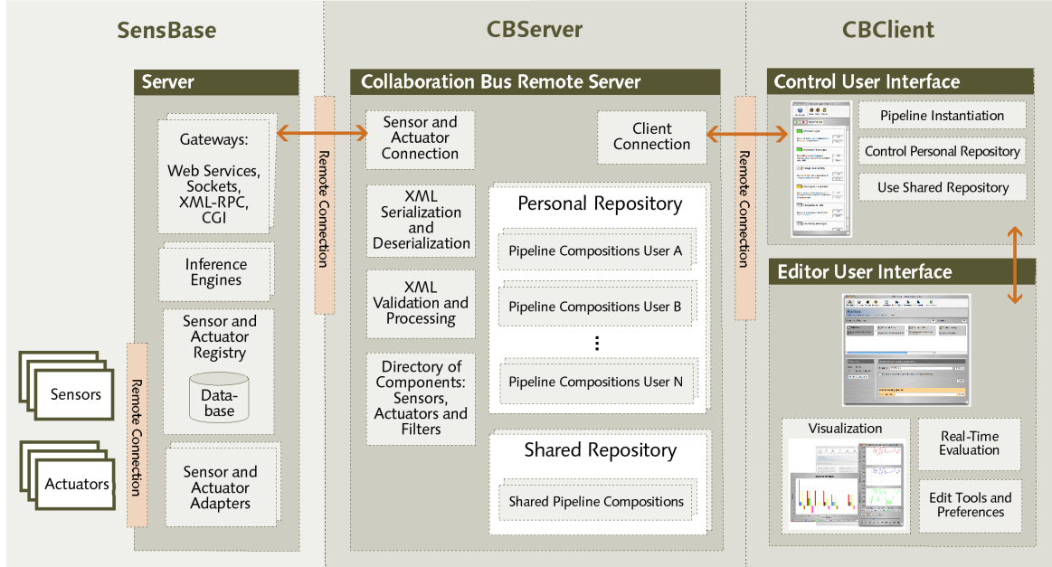
Figure 6. CollaborationBus software architecture.
