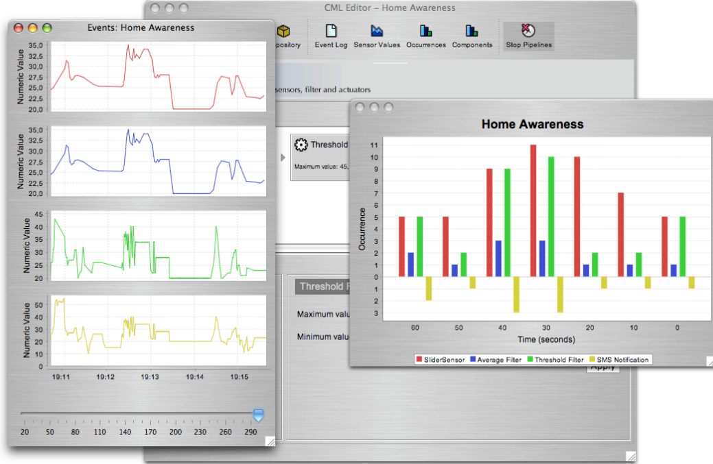
Figure 5. Real-Time Visualisation GUI (with time plot visualization, and overview of the pipeline events).
