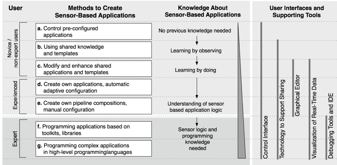
Figure 1. User experience levels, and adequate tools to support users.
