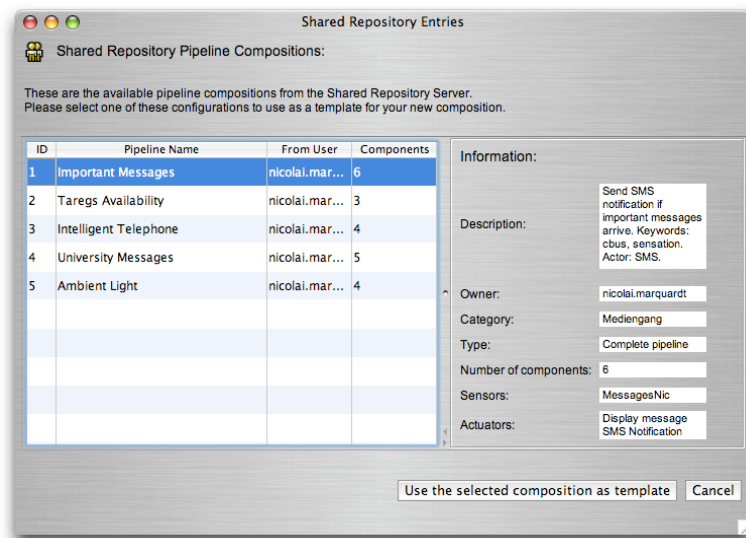
Figure 4. Shared Repository GUI.
