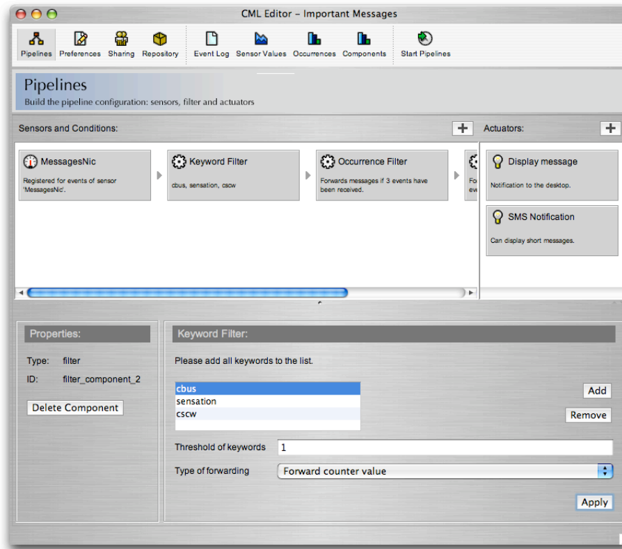
Figure 3. Editor GUI.
